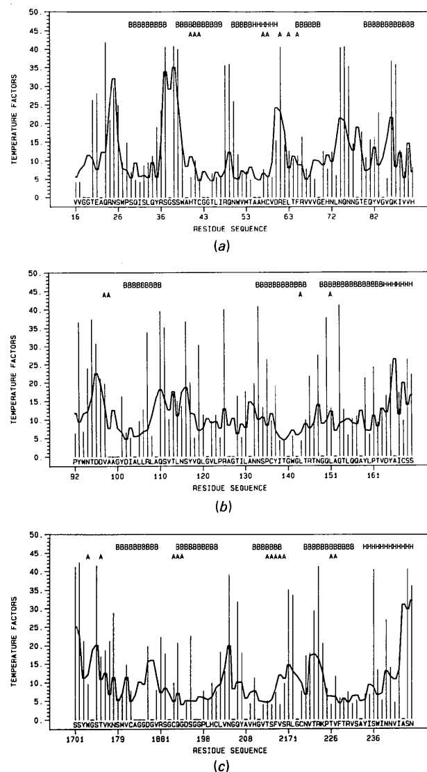
Fig. 1. Plot of isotropically refined temperature factors [ B(\text{Å}^2) ], side-chain (bar) and backbone (continuous plot) atoms as a function of sequence number (according to chymotrypsinogen) with amino acids indicated by the appropriate letter. Above the plot, secondary structure is indicated: H for helix, B for \beta structure. Amino acids involved with substrate binding ( S4 to S2' subsites, Table 2) are marked with an A .
