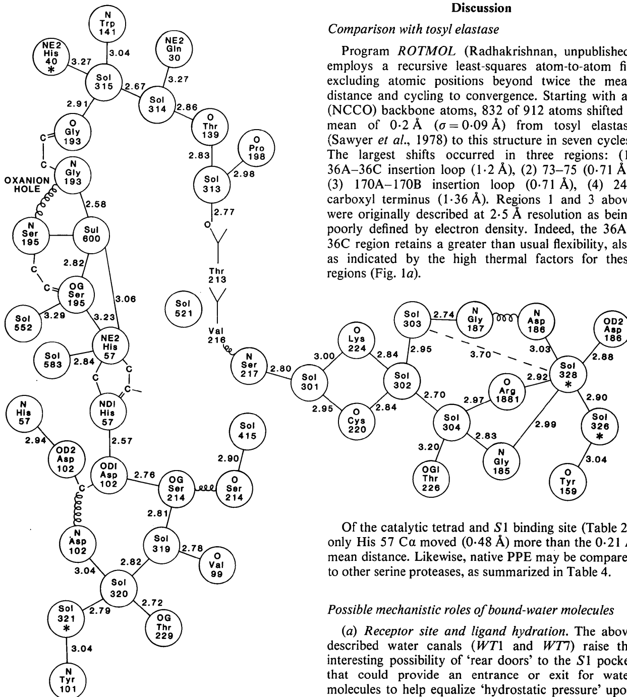
Fig. 5. A topological view of active-site residues and water channels WT1 , WT4 and WT7 is given, together with bond lengths of hydrogen bonds. The sulfate (600) ion is also shown. Surface water molecules are marked with an asterisk.
