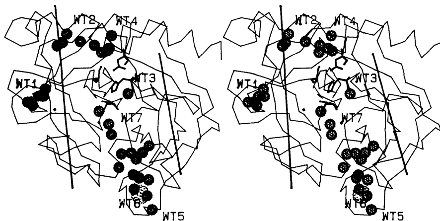
Fig. 2. Stereoview of \alpha -carbon backbone of PPE, looking towards the catalytic tetrad, with the S and S' regions of the extended binding site to the left and right, respectively. Vectors are drawn to represent the centers of the \beta -barrel domains. Seven water domains are drawn and labelled (WT1–WT7).
