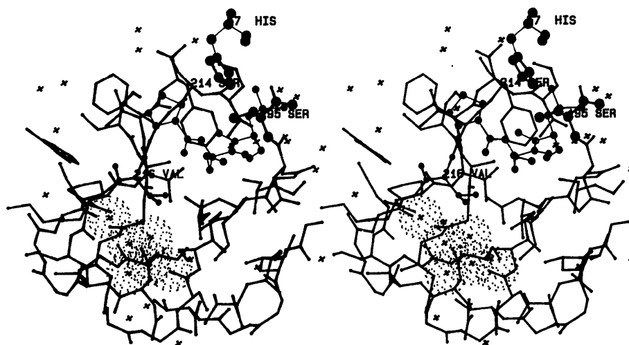
Fig. 3. Stereoview of the WT1 internal bound-water region of PPE in approximately the same orientation as Fig. 2. A portion of the hexapeptide (Pro-norvaline- N -methylleucine; Meyer et al. , 1987) is shown in binding sites S2 – S1 – S1' , drawn with small balls for atoms and thin lines for bonds. Ser 195 and His 57 of the catalytic triad are drawn as larger balls and labelled. Van der Waals' surfaces are used to illustrate the size and shape of this water tunnel that extends into the 'left' \beta -barrel at the back of the S1 primary specificity site.
