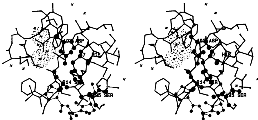
Fig. 4. Buried water channel, WT4 , connecting the catalytic tetrad with bulk solvent, is illustrated in this stereoview. As in Fig. 3, the tripeptide is shown bound to the receptor sites S2–S1–S1'. The catalytic tetrad is drawn with larger balls representing individual atoms. The water molecules Sol 319–320–321 are drawn with van der Waals' radii, illustrating the size and shape of the tunnel.
