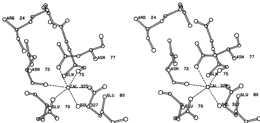
Fig. 6. Stereoview of the calcium binding site in PPE.
