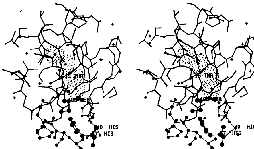
Fig. 7. As with Figs. 3 and 4, a tripeptide is drawn (small balls) into the active site; the catalytic tetrad is drawn as larger balls. The buried water channel is bounded by interior Thr 213 and His 40 on the surface. The norvaline side chain (Meyer et al. , 1987) is inserted into the S 1 pocket; the Thr 213 side chain may act as a pivot, permitting water molecules to be expelled from (or to enter) the S 1 pocket upon ligand binding.
